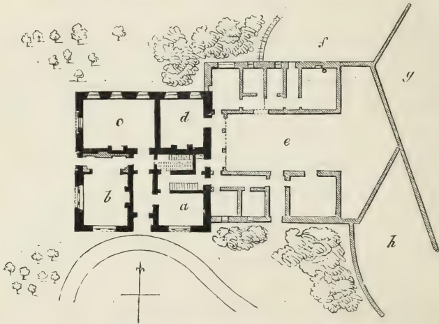
[Fig. 108. Ground-plan of the Villa at Brentry Hill.]
